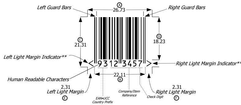
Nominal size (Magnification 100%) EAN-8 bar code symbol illustration
